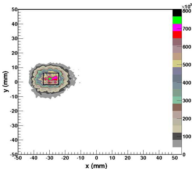
Figure 9. Integrated charge profile (in fC) as a function of WCE coordinates for a four anode PMT (R7600U-100-M4). Black rectangle shows the selection cut applied in order to include the signal from the fiber bundle only.
