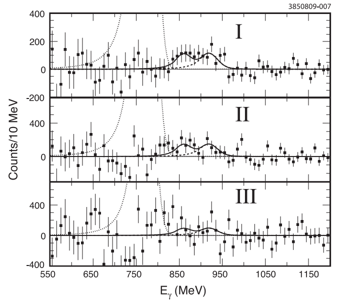
FIG. 2. Background- and \chi_{bj}(2P) -subtracted distributions of E_\gamma from Y(3S) decays in three |\cos \theta_T| regions, I, II, and III defined in the text. The curves are the results of the joint fit, with a CL of 18.5%. The \chi_{bj}(2P) peaks are indicated by the dotted lines and the \eta_b signals by the dashed lines, which join the solid line.
