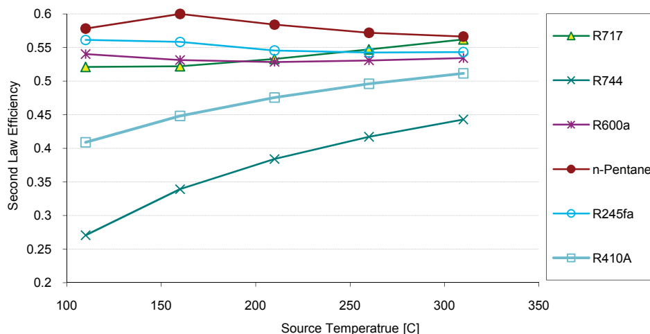
Figure 7: Comparison of the Second Law efficiency as a function of source temperature for the ORC with Zerol-flooded expansion and internal regeneration.
