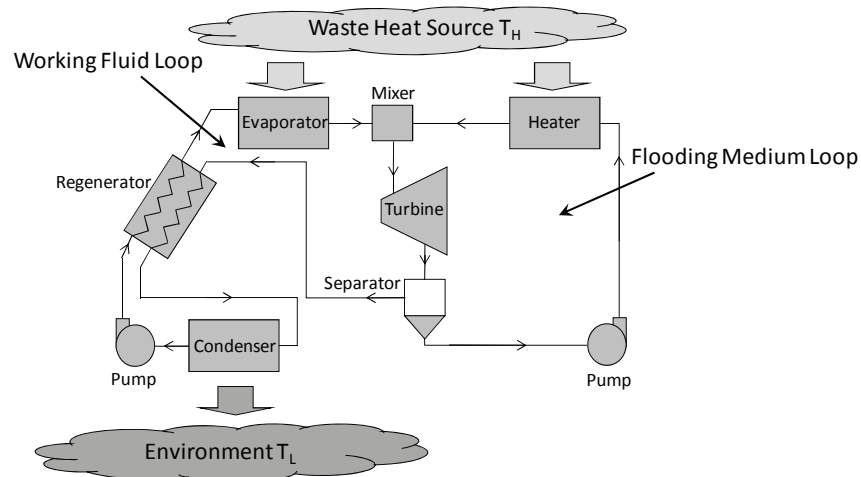
Figure 1: Schematic diagram showing the ORC with internal regeneration. The working fluid cycles through the left-hand loop, while the flooding medium cycles through the right-hand loop. Both fluids flow together through the turbine.
