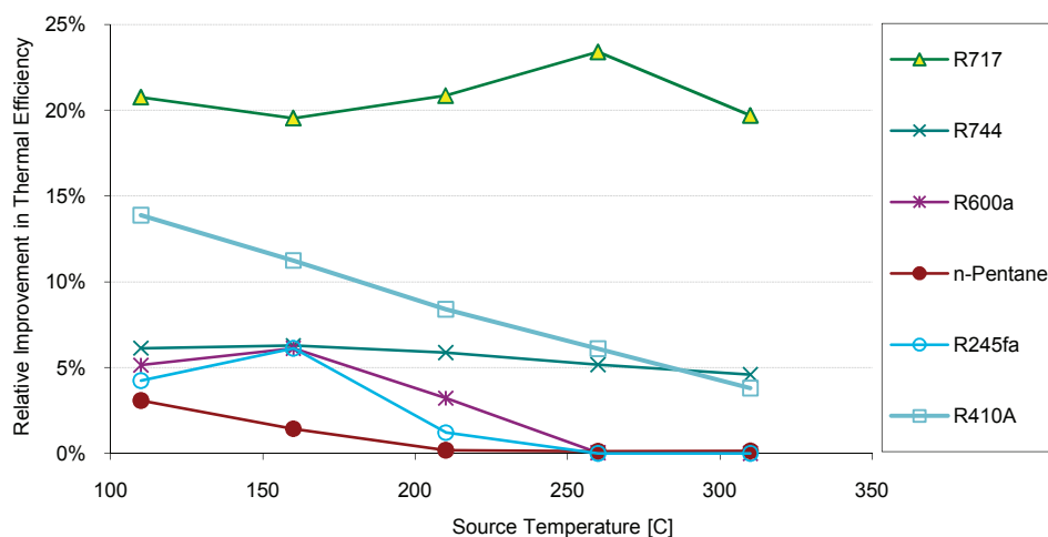
Figure 6: Comparison of the improvement in thermal efficiency as a function of source temperature for the ORC with water-flooded expansion and internal regeneration relative to the ORC with internal regeneration only.
