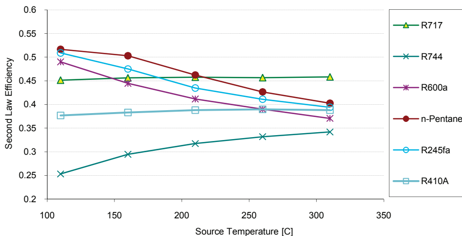
Figure 2: Comparison of the Second Law efficiency for the baseline ORC as a function of source temperature for all working fluids studied.
