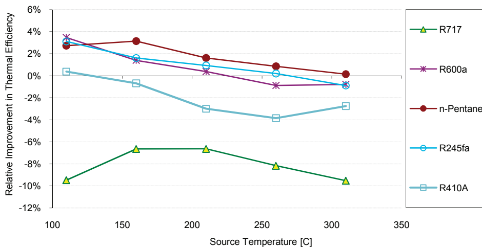
Figure 9: Comparison of the improvement in thermal efficiency as a function of source temperature for the ORC with one open feedwater heater and internal regeneration relative to the ORC with Zerol-flooded expansion and internal regeneration. (R744 has been omitted because its critical point is too low for an effective feedwater heater to be implemented.)
