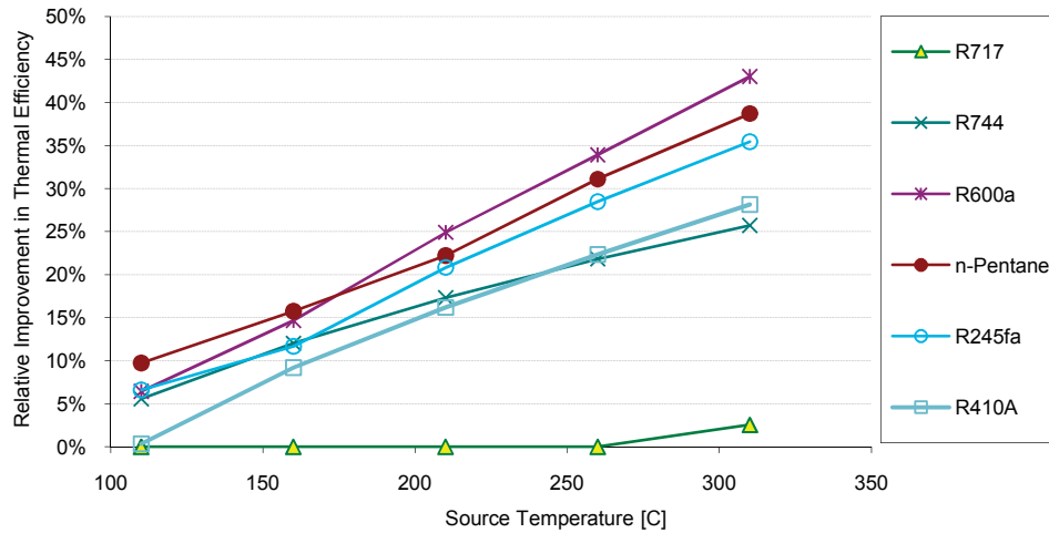
Figure 4: Comparison of the improvement in thermal efficiency as a function of source temperature for the ORC with internal regeneration relative to the baseline cycle.
