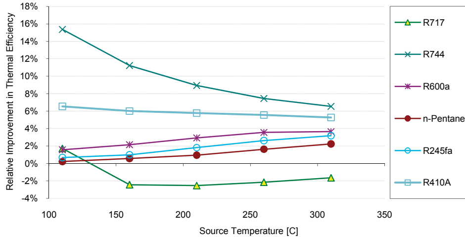
Figure 8: Comparison of the improvement in thermal efficiency as a function of source temperature for the ORC with one reheat stage and internal regeneration relative to the ORC with Zerol-flooded expansion and internal regeneration.
