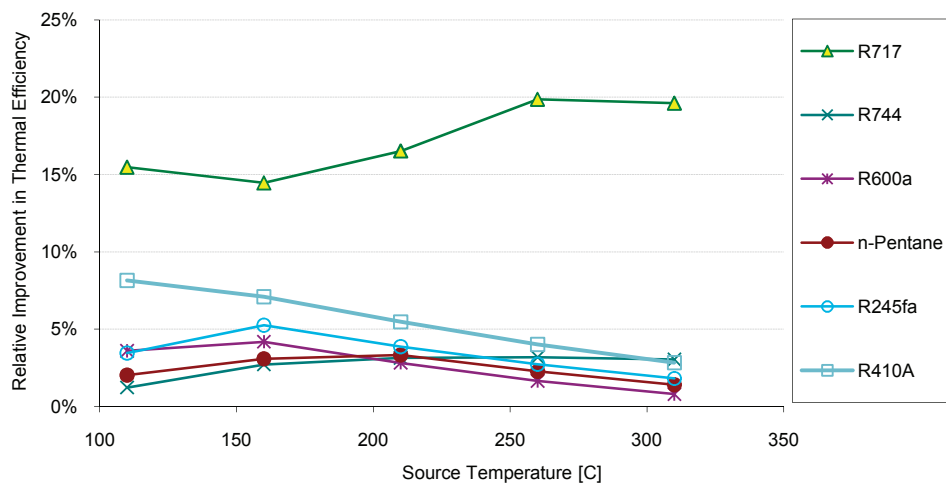
Figure 5: Comparison of the improvement in thermal efficiency as a function of source temperature for the ORC with Zerol-flooded expansion and internal regeneration relative to the ORC with internal regeneration only.
