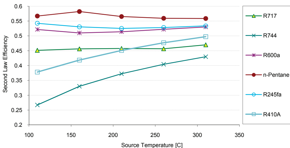
Figure 3: Comparison of the Second Law efficiency as a function of source temperature for the ORC if only internal regeneration is applied.
