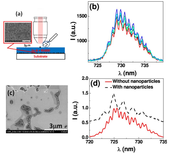
Fig. 2. (Color online) (a) Schematic illustration of our optical setup. Inset, SEM image of randomly distributed silica nanoparticles on a glass substrate before applying SU-8 polymer on it. (b) Spectra of random lasing emission from the random laser film measured over time. Each acquisition time is 1 s averaged over \sim 500 pumping pulses. (c) SEM image of silica nanoparticles attached to the top of the random laser film. (d) Changes in the emission spectrum before (red solid line) and after (black dashed line) introducing the nanoparticles.
