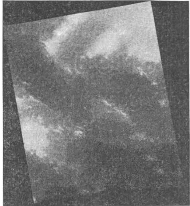
Figure 3: Phoenix West Elevation Image. Digital terrain information for the Phoenix West quad is shown here as a brightness image i.e., the brighter the image, the higher the elevation. This data has been corrected to register with the Landsat quad with an accompanying pixel change to 80 meters.
