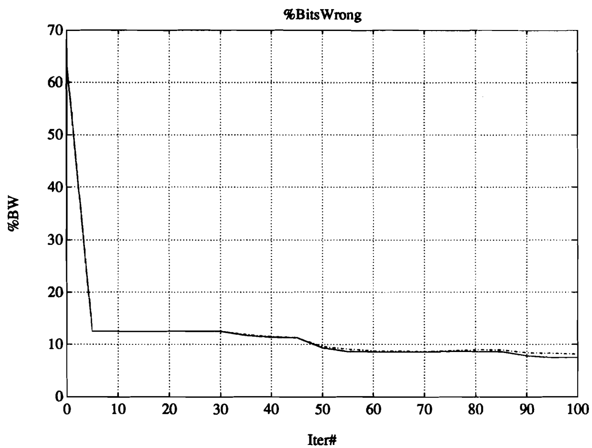
Figure 1.6 A sample 'percent bits wrong' graph, generated by the mbckprop program, is shown here. The solid line is the training percent bits wrong and the dashed line is the testing percent bits wrong.
