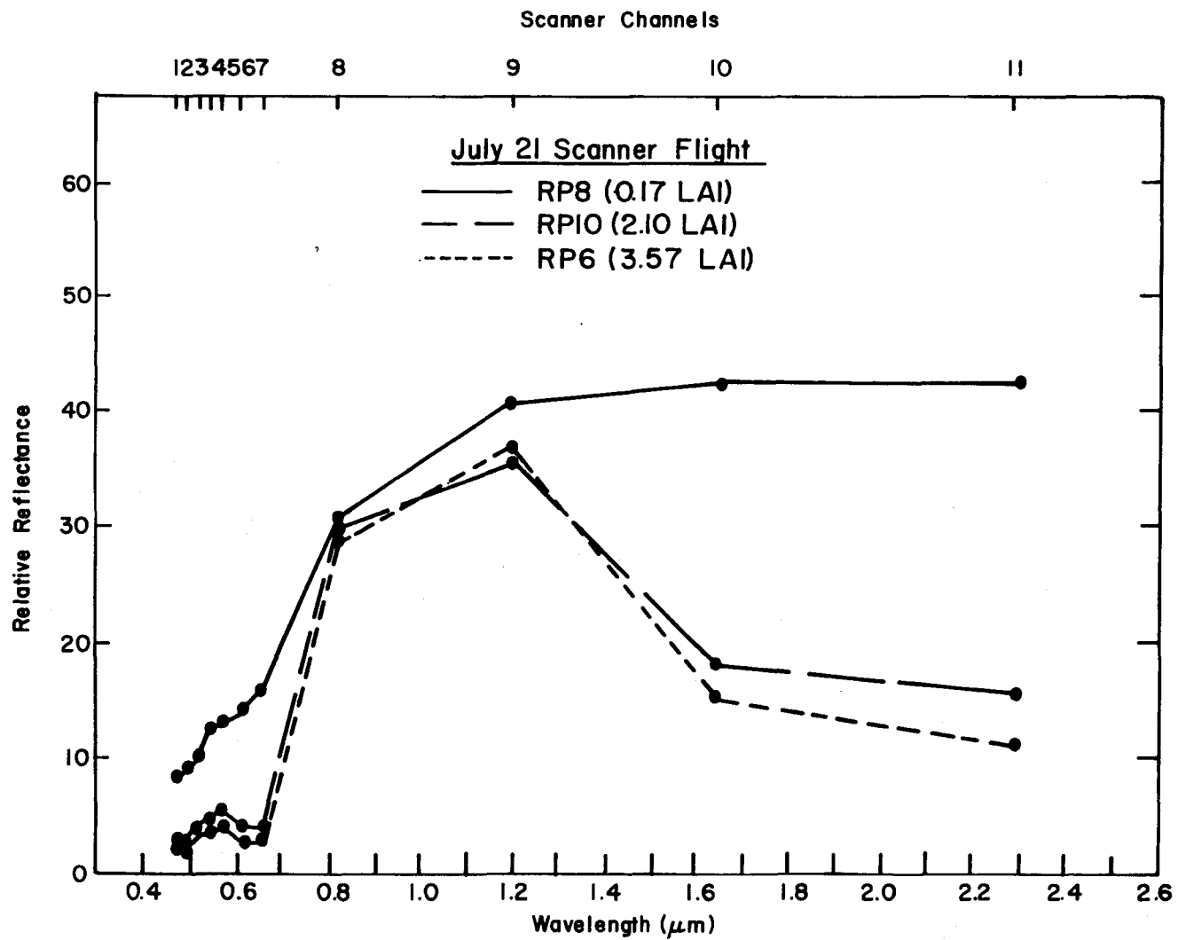
Figure 6. Normalized spectral response curves for three Russell plots, July 21.
