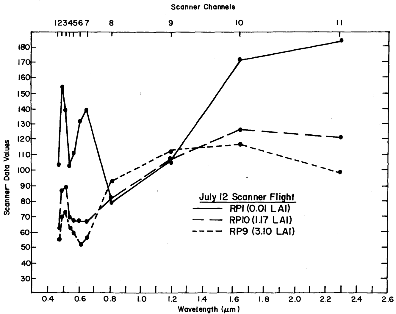
Figure 4. Uncalibrated scanner response curves for three Russell plots, July 12.
