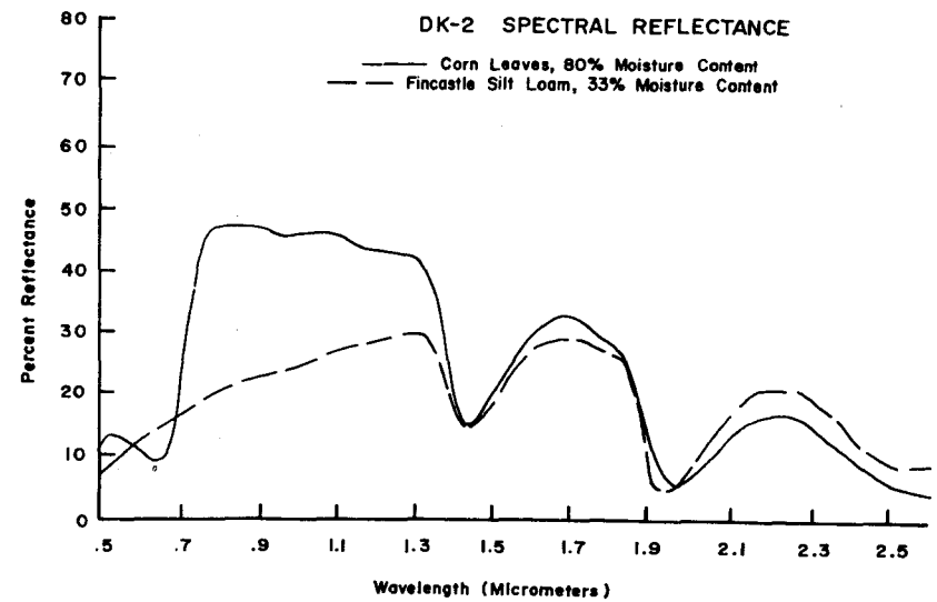
Figure 3. DK-2 spectral reflectance of maize leaves and of two soils in air dry and saturated conditions.
