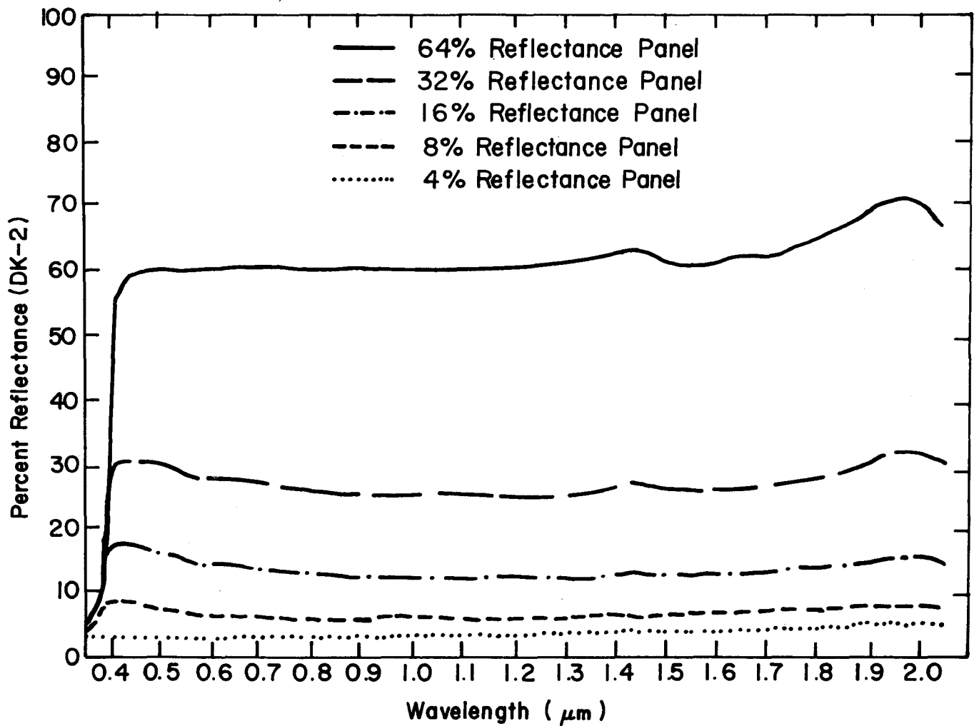
Figure 2. DK-2 spectral reflectance for five LARS gray scale panels.
