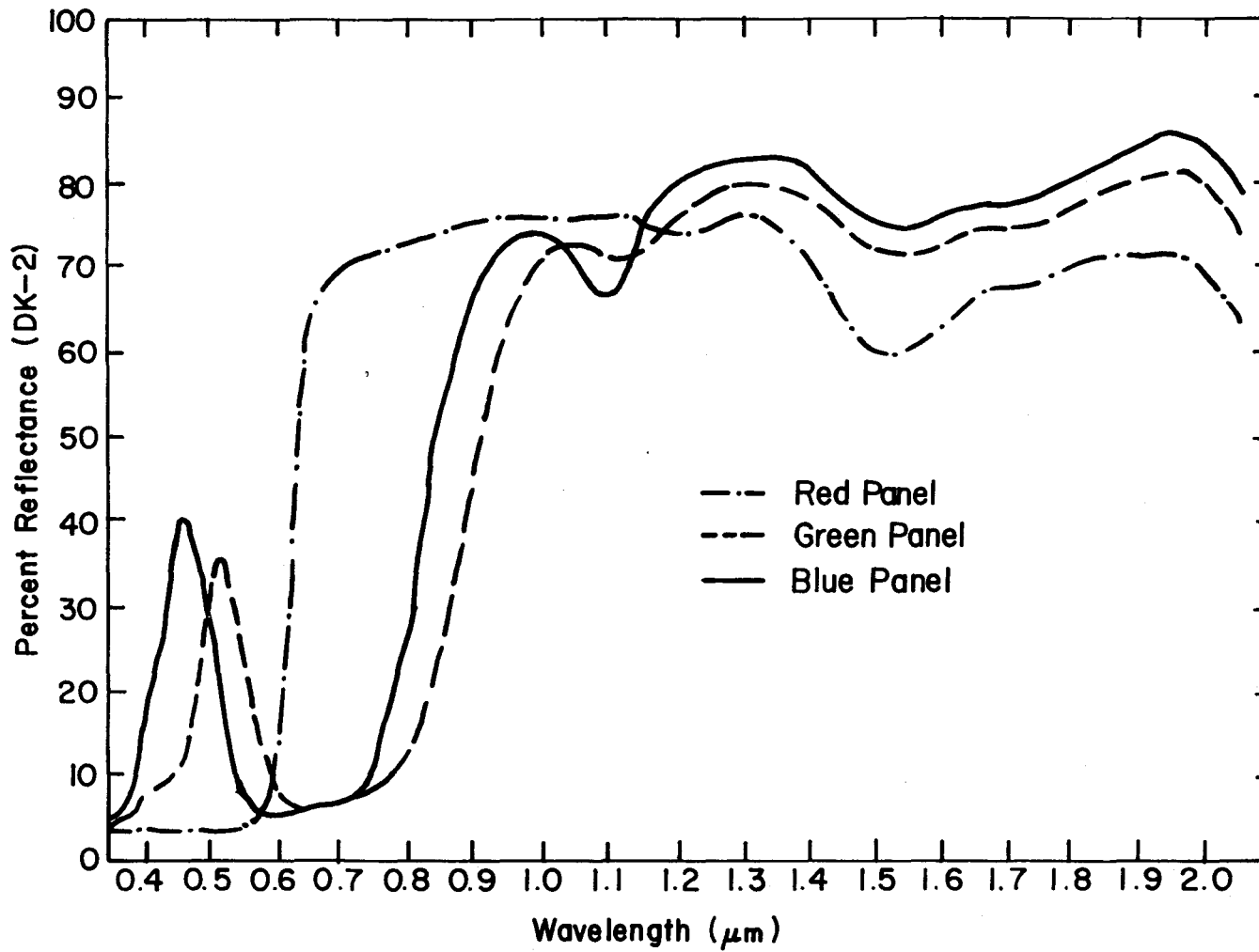
Figure 1. DK-2 spectral reflectance for red, green, and blue LARS color panels.
