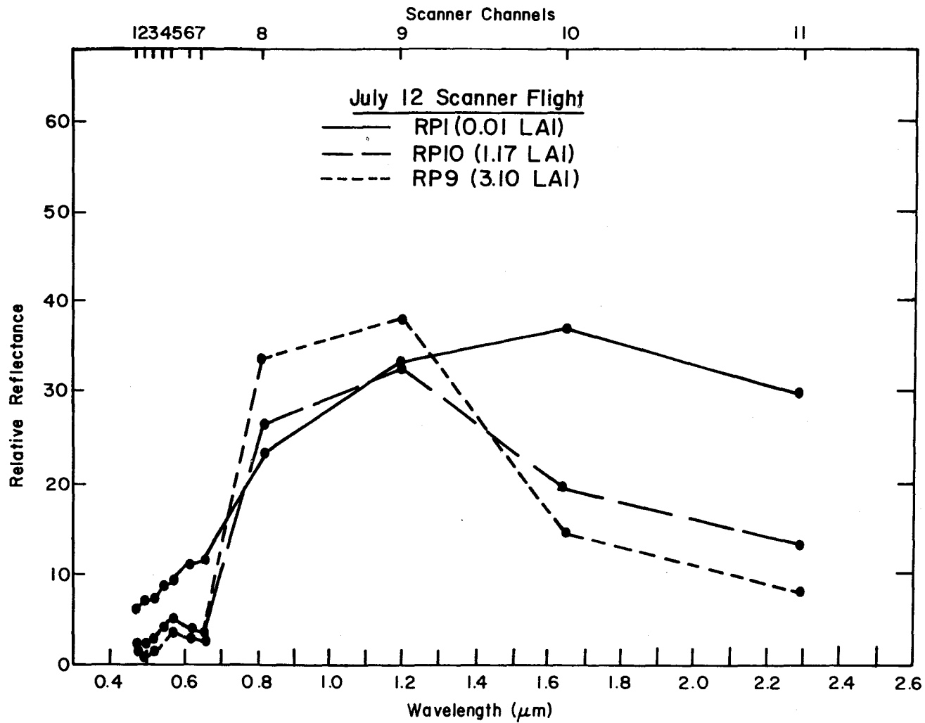
Figure 5. Normalized spectral response curves for three Russell plots, July 12.
